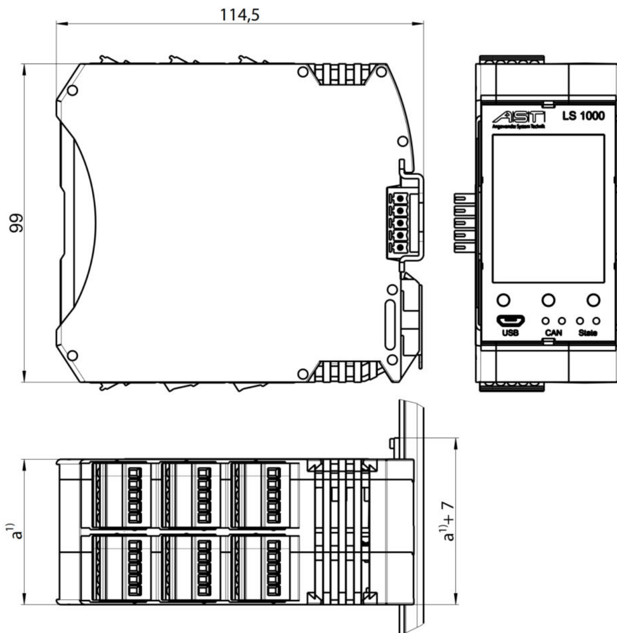
Figure 1 - Dimensions LS 1000
