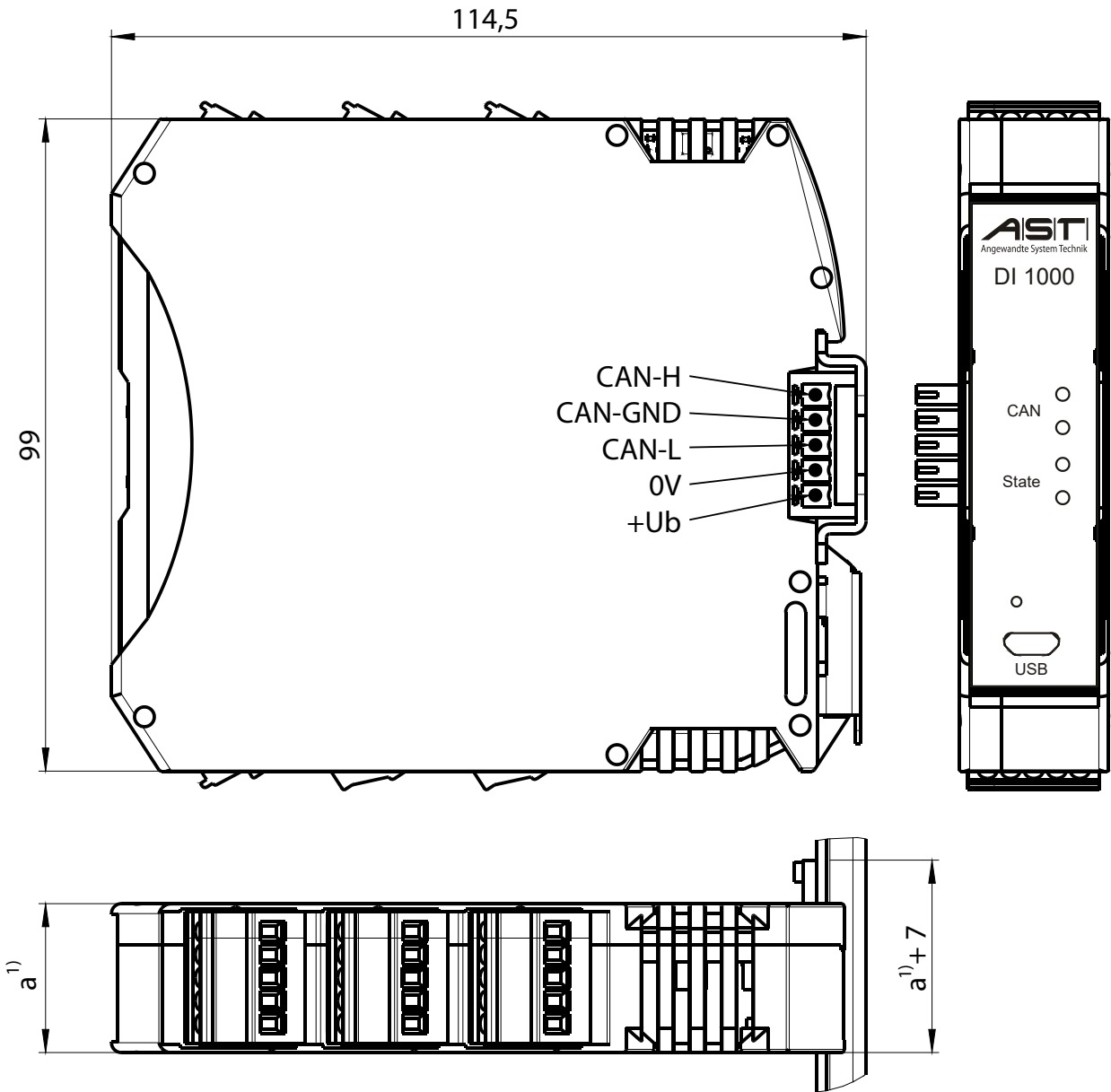
1) - see type code Figure 1 - Dimensions DI 1000
